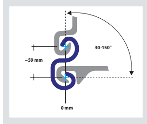
LV20n Larssen / Z
