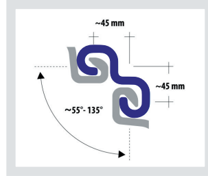
LVO (Omega) Larssen / Z
