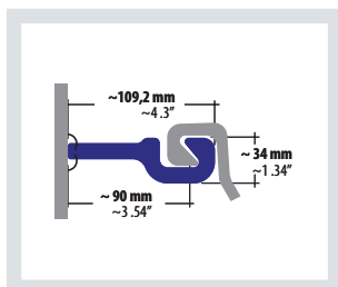
LPB180 Larssen / Z
