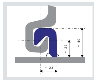
E-21 Larssen / Z
